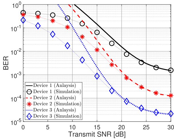
Fig. 5. BER of the uplink IM-NOMA system with imperfect CSI when L = 3 , (S, K) = (4, 1) , N = 2 , (M_1, M_2, M_3) = (4, 2, 2) , (d_1, d_2, d_3) = (2, 1.5, 1) , and \sigma_e^2 = 0.01 .
