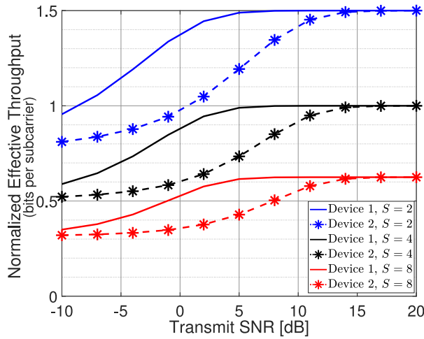
Fig. 6. Normalized effective throughput of the uplink IM-NOMA system with the JML detector for a various number of available subcarriers S = 2, 4 and 8 when L = 2 , N = 4 , M = 4 , K = 1 , and (d_1, d_2) = (1, 2) .
