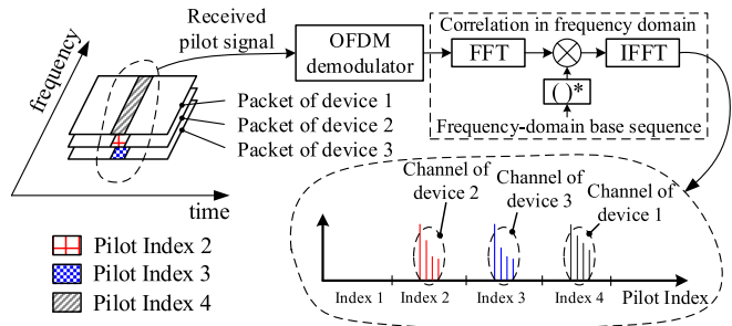
Fig. 2. Implementation of the decomposition of uplink pilot signals.
