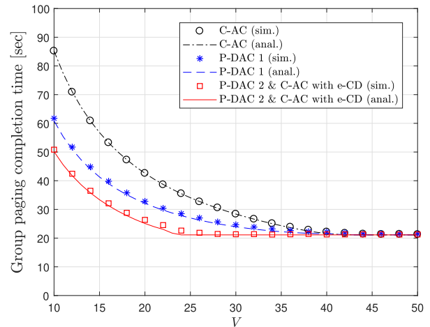
Fig. 8. GPC time of the proposed DAC mechanisms for varying the number of PUSCH resources ( V ).
